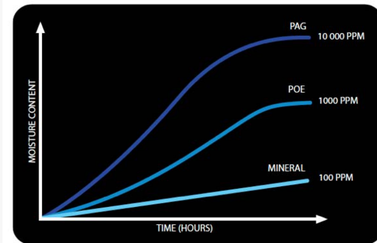
Hygroscopy of POE and mineral lubricants
